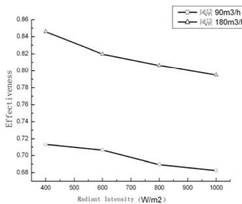
Fig.8 Plots of simulation results in the form of Effectiveness vs. Radiant Intensity
