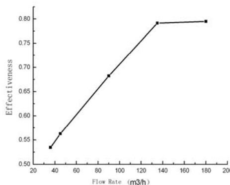
Fig. 6 Plots of simulation results in the form of Effectiveness vs. Flow rate
