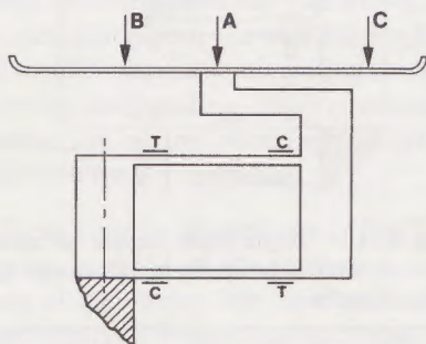
Fig. 2.8 — Dual-beam spring element for reduced sensitivity to off-axis loads.
