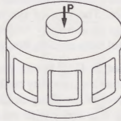
Fig. 2.27 — Slotted-cylinder, multiple-column configuration for high-capacity, low-profile applications.
