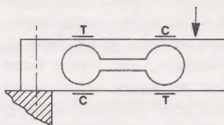
Fig. 2.9 — Popular "binocular" spring element, widely used in low-capacity scale applications.
