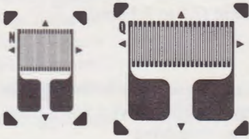
Fig. 4.2 — Typical single-element grid patterns for transducer applications.
