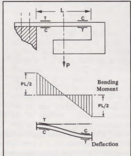
Fig. 2.5 — Reversed bending induced by folded cantilever beam.
